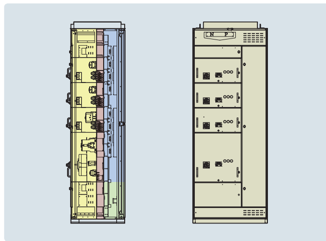
480V MCC
