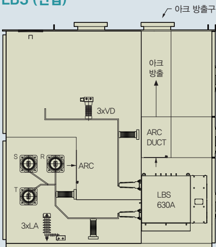
LBS (인입)
