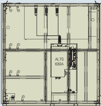
ALTS (인입)
