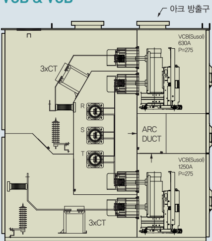
VCB & VCB
